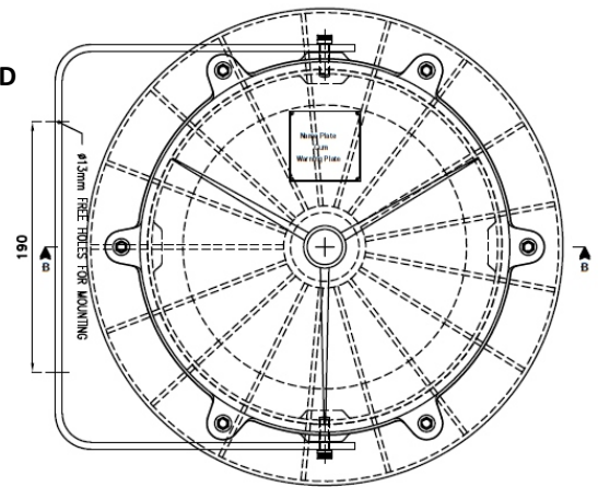
Plan View of Well Glass Fitting (TYPE - Z)
